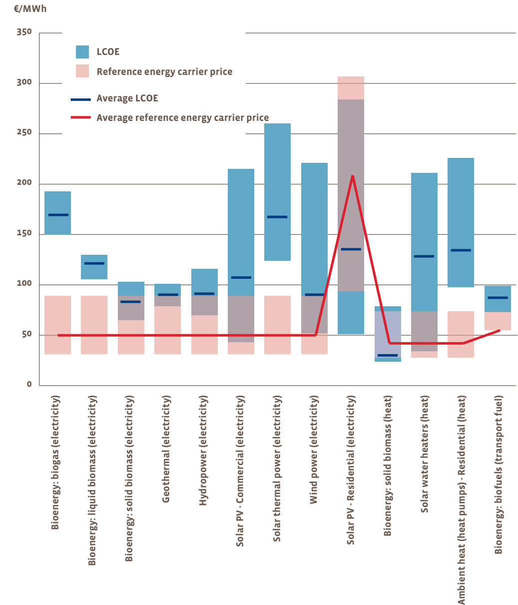
LCoE and reference energy carrier (€/MWh) EU Overview
