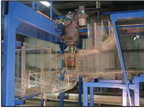
Figure 1. Left: U.S. Army Corps of Engineers Engineering Research and Development Center (ERDC) hydraulic observational turbine model (1:25 scale) for the Ice Harbor runner replacement project. Photo credit: USACE. Right: Computational fluid dynamics (CFD) model used to predict the probability of fish passage through various regions of the turbine. Photo credit: USACE.
