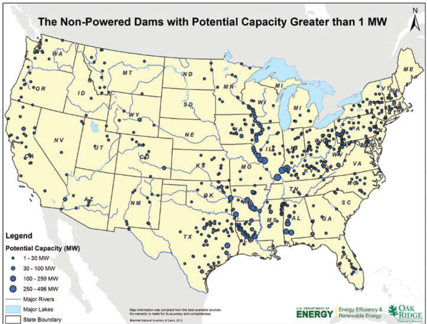
Figure 5. Location of the top non-powered dams in the United States with potential capacities greater than 1 MW.
