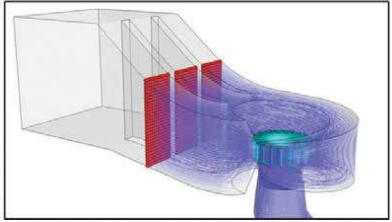
Figure 1. Left: U.S. Army Corps of Engineers Engineering Research and Development Center (ERDC) hydraulic observational turbine model (1:25 scale) for the Ice Harbor runner replacement project. Photo credit: USACE. Right: Computational fluid dynamics (CFD) model used to predict the probability of fish passage through various regions of the turbine. Photo credit: USACE.
