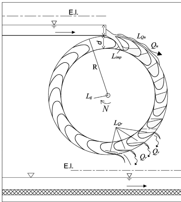
Fig. 5. Sketch of an overshot water wheel with radius R , rotational speed N , bucket depth d , lost flow rates Q_u and Q_r , and power losses L [52]. E.I. is the head energy line. Power losses are described in Section 3.3.
