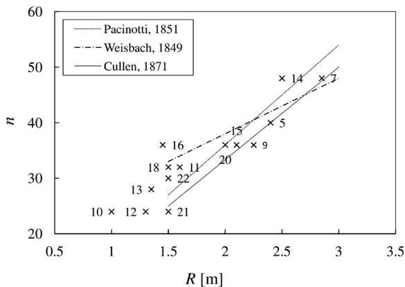
Fig. 6. The number of blades proposed by Pacinotti [54], Weisbach [48] and Cullen [55] as a function of the radius R (overshot water wheels). The three design laws give similar results. Data of real overshot water wheels are also depicted, with reference to the wheel number reported in Table 5.
